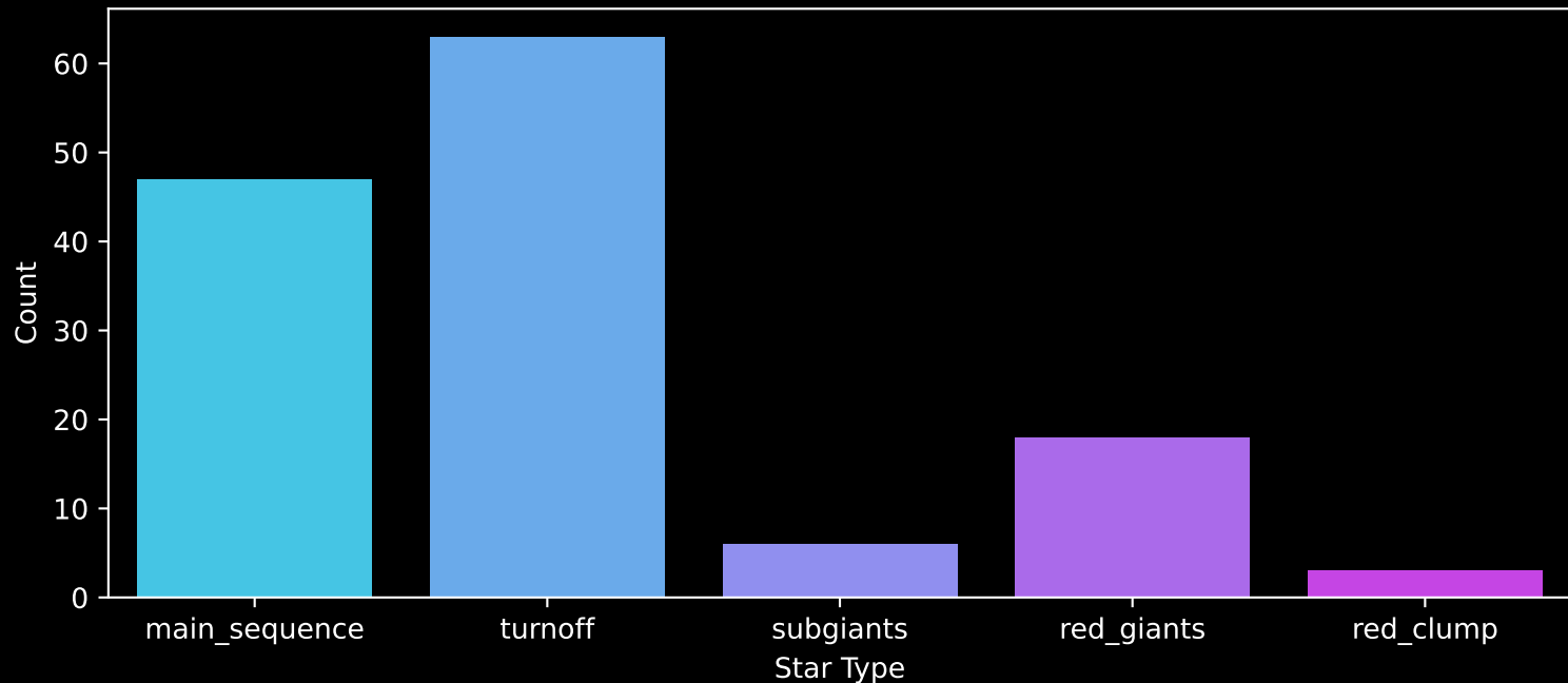
APOGEE DR17 Field: [ORIONB-RV_btx] Count plot of Star Type
