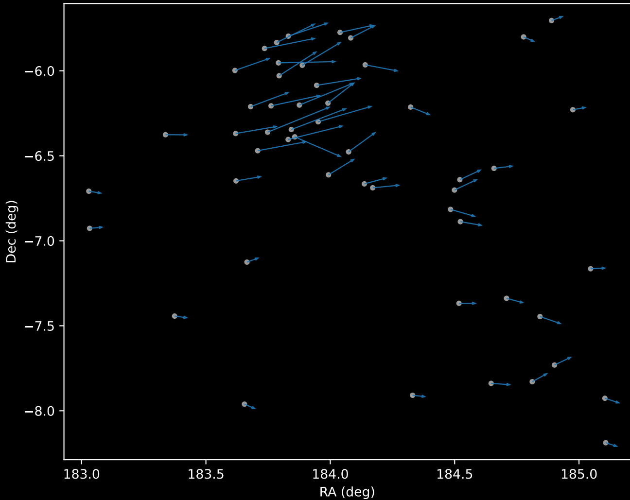
APOGEE DR17 Cluster 0 Proper Motion Vectors (n=52)
