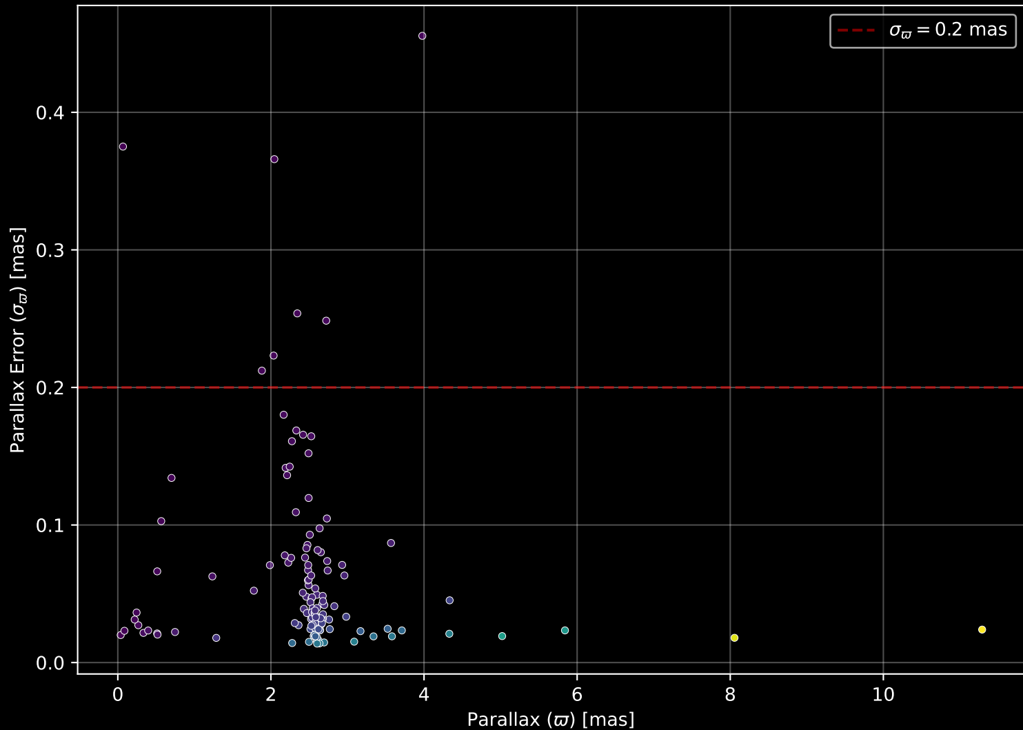
APOGEE DR17 Field: [ORIONB-RV_btx] Parallax Quality (n= 137)
