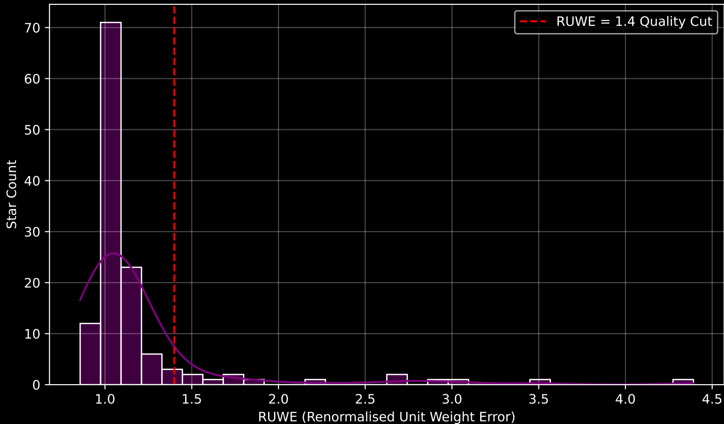
GAPOGEE DR17 Field [ORIONB-RV_btx] RUWE Distribution (n= 128)
