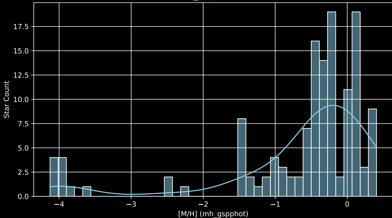
APOGEE DR17 Field: [ORIONB-RV_btx [M/H] (mh_gspphot) (n= 137)
